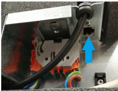
Figur 12: Ethernet-tilkobling, RJ45
